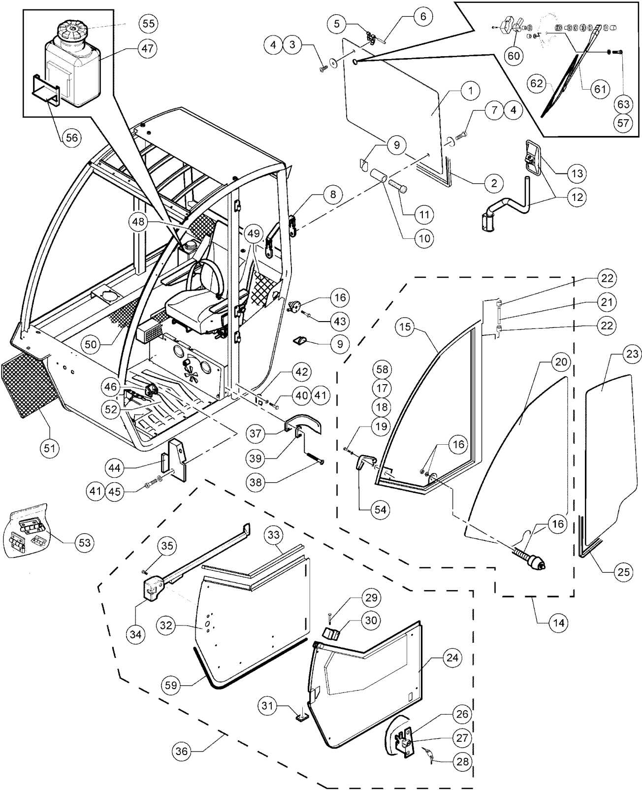
402.1 607476 Cabin - View 2
